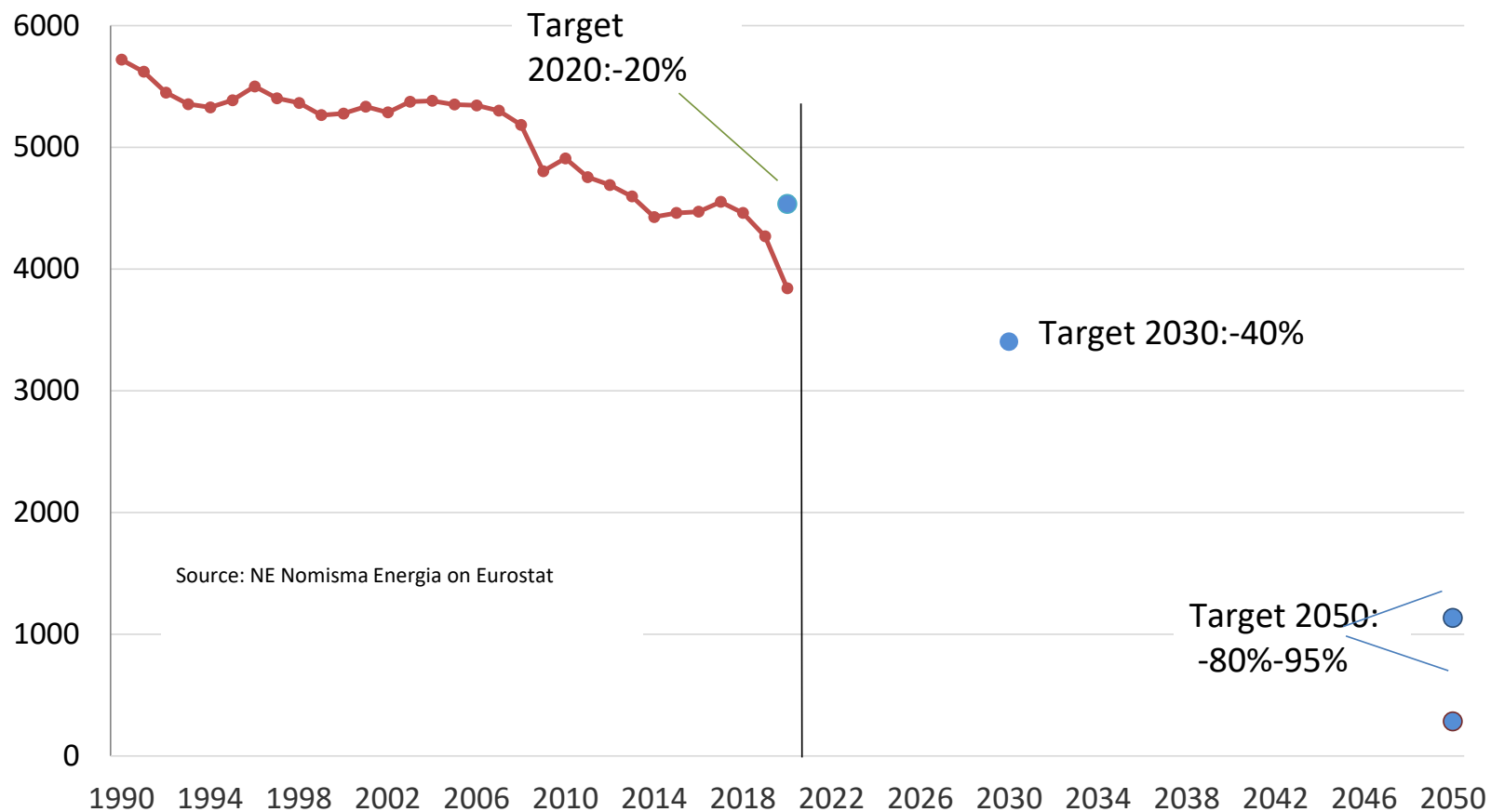
European Union CO2 emission; actual and targets Milion tons
