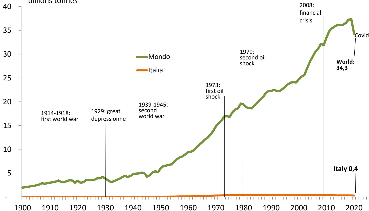
120 years of CO2 emissions from fossil fuels billions tonnes
